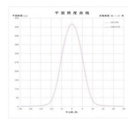
500W照度图 500W Illumination curve
