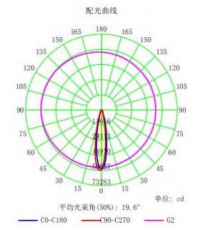
100W配光曲线 100W Light distribution curve
