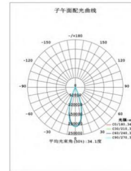
500W配光曲线 500W Light distribution curve
