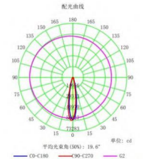
100W配光曲线 100W Light distribution curve
