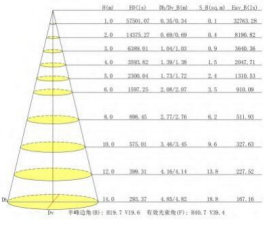
100W照度图 100W Illumination curve
